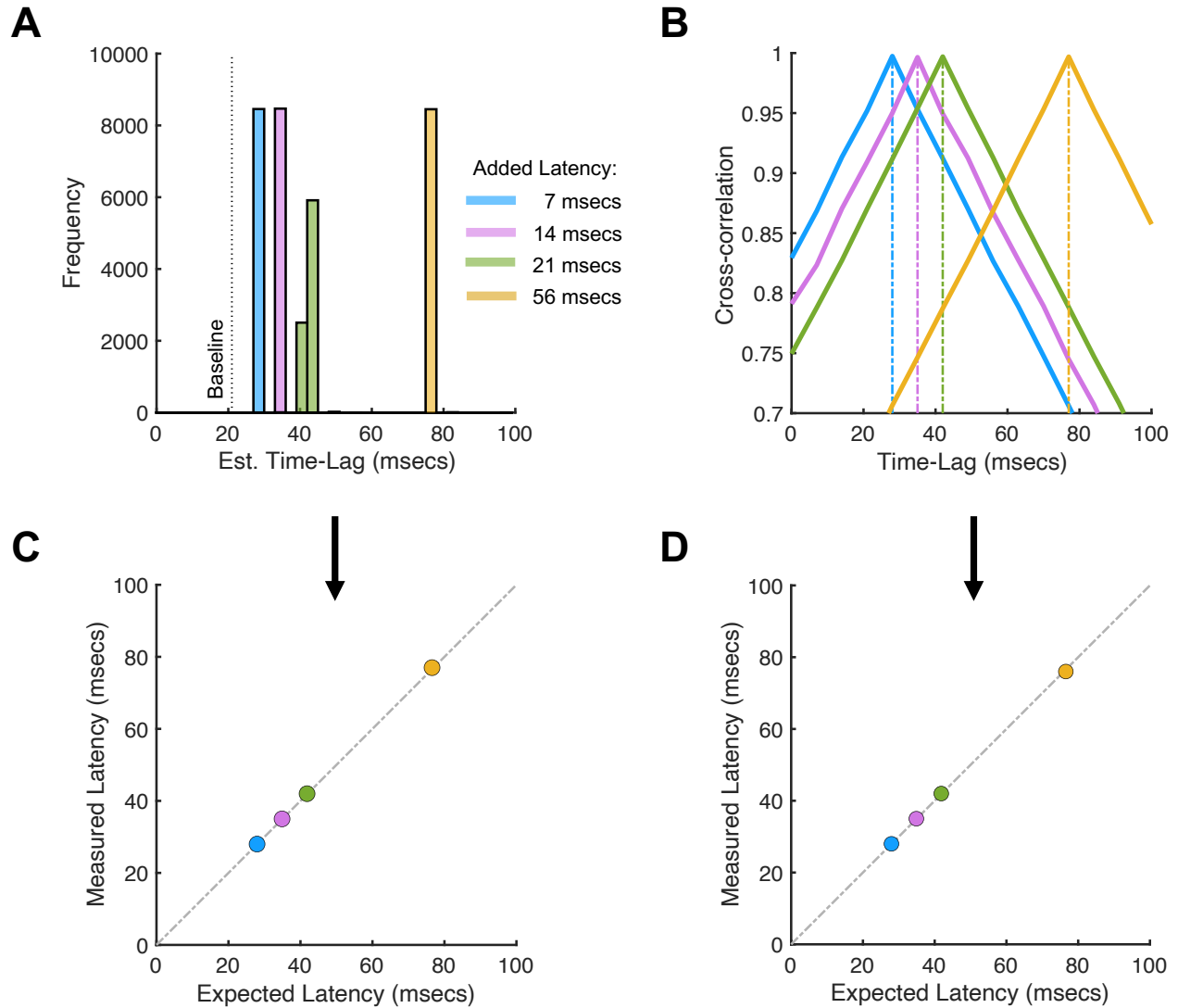
Figure 4. Agreement between measured and expected system latencies. (A) Histogram of measured latencies for various amounts of additional latency that was added programmatically. (B) Cross-correlation between left and right pupil velocities over a range of time-lags. Position data are omitted, but produced the same maxima. (C) Median latencies, based on the distributions in (A), as a function of known system latency. The dashed diagonal line indicates perfect measurement accuracy. Standard deviation error-bars are plotted but are smaller than the markers. (D) Time-delays in (B) that produced the cross-correlation maxima, plotted as a function of known system latency.
